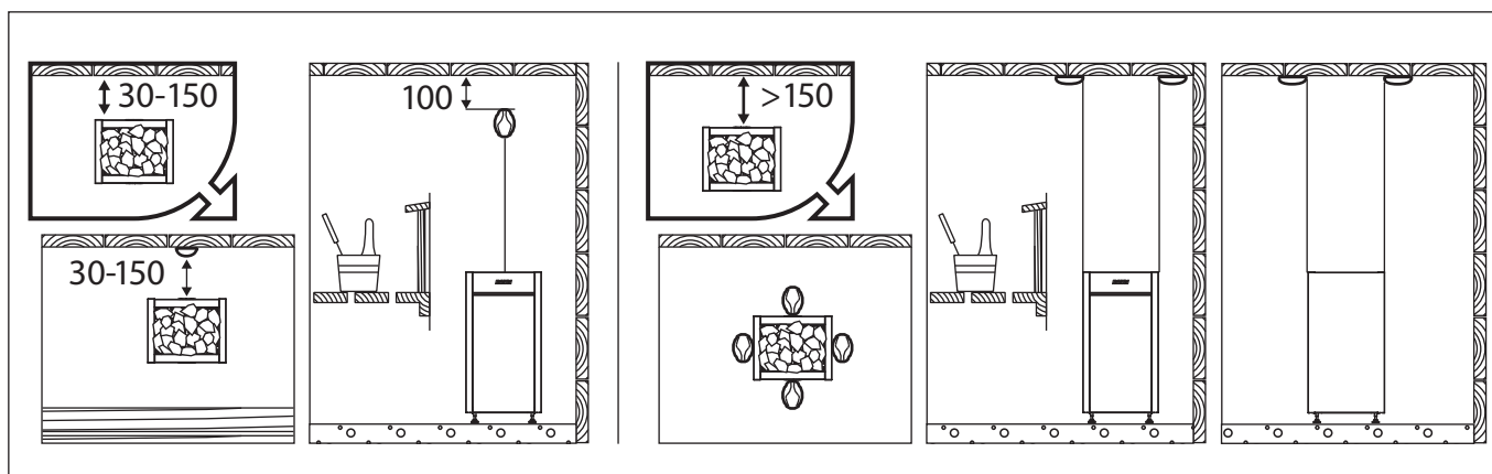
Installing the sensor (all dimensions in millimeters)
