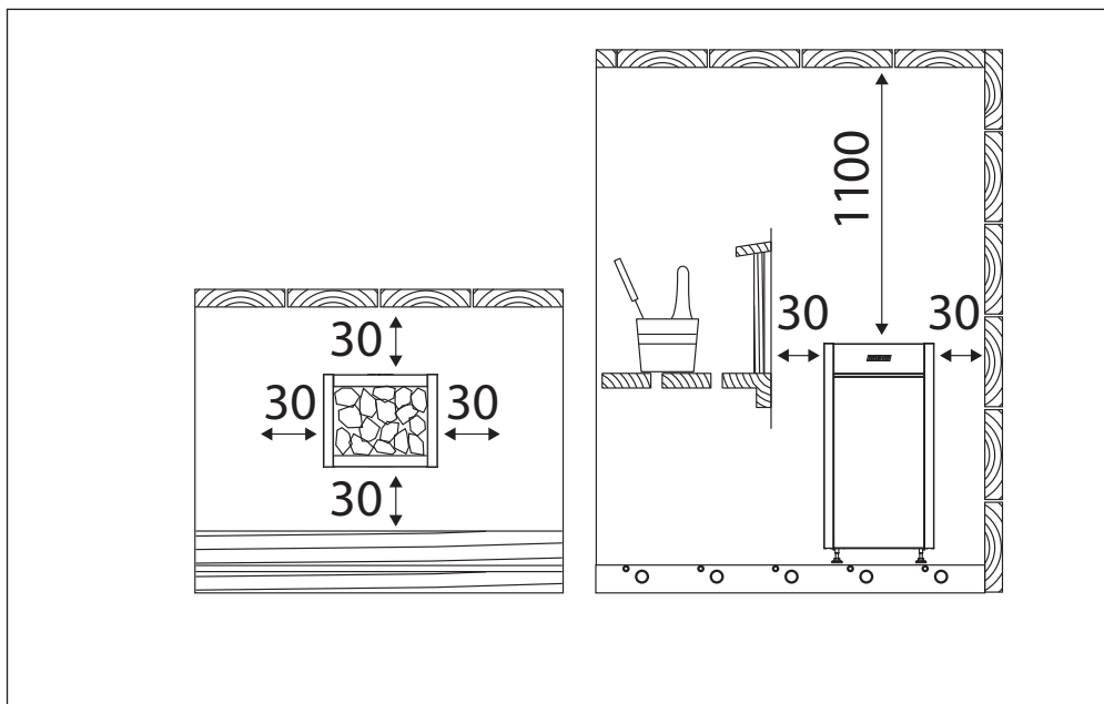
Minimum safety distances (all dimensions in millimeters)
