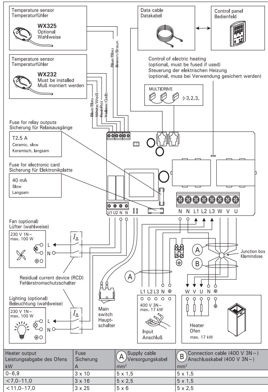
Electrical connections of control unit CG170 and HL heater
