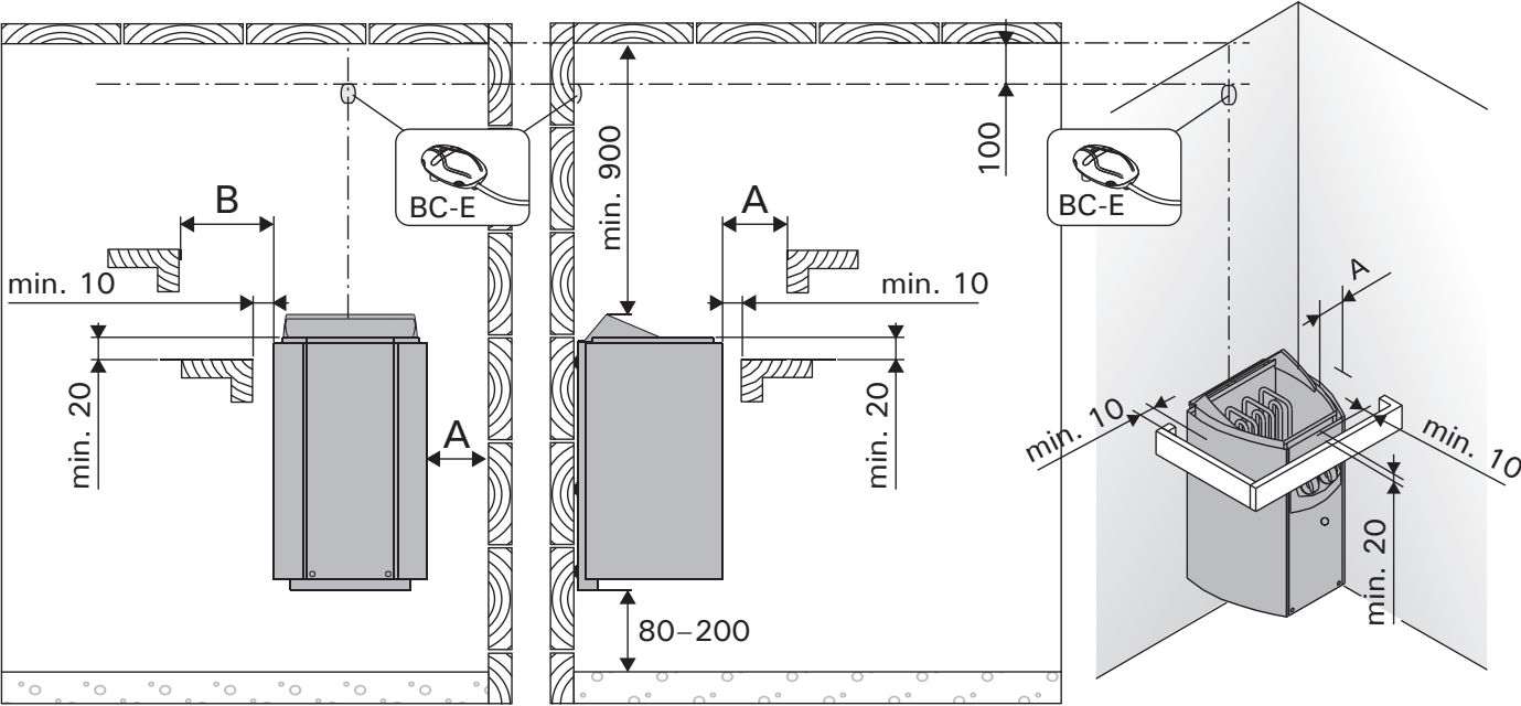
Safety distances (all dimensions in millimeters)
