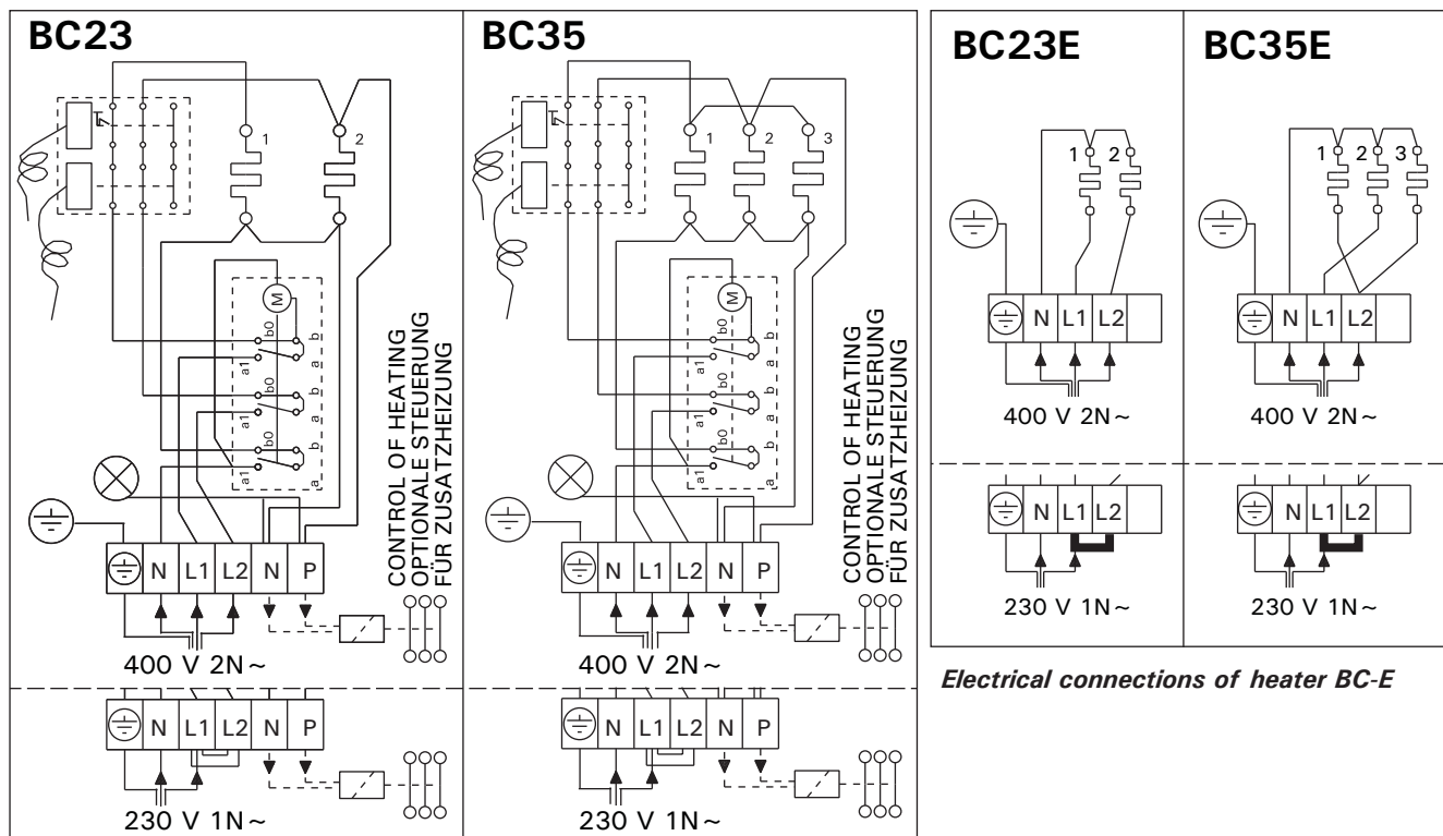
Electrical connections of heater BC
