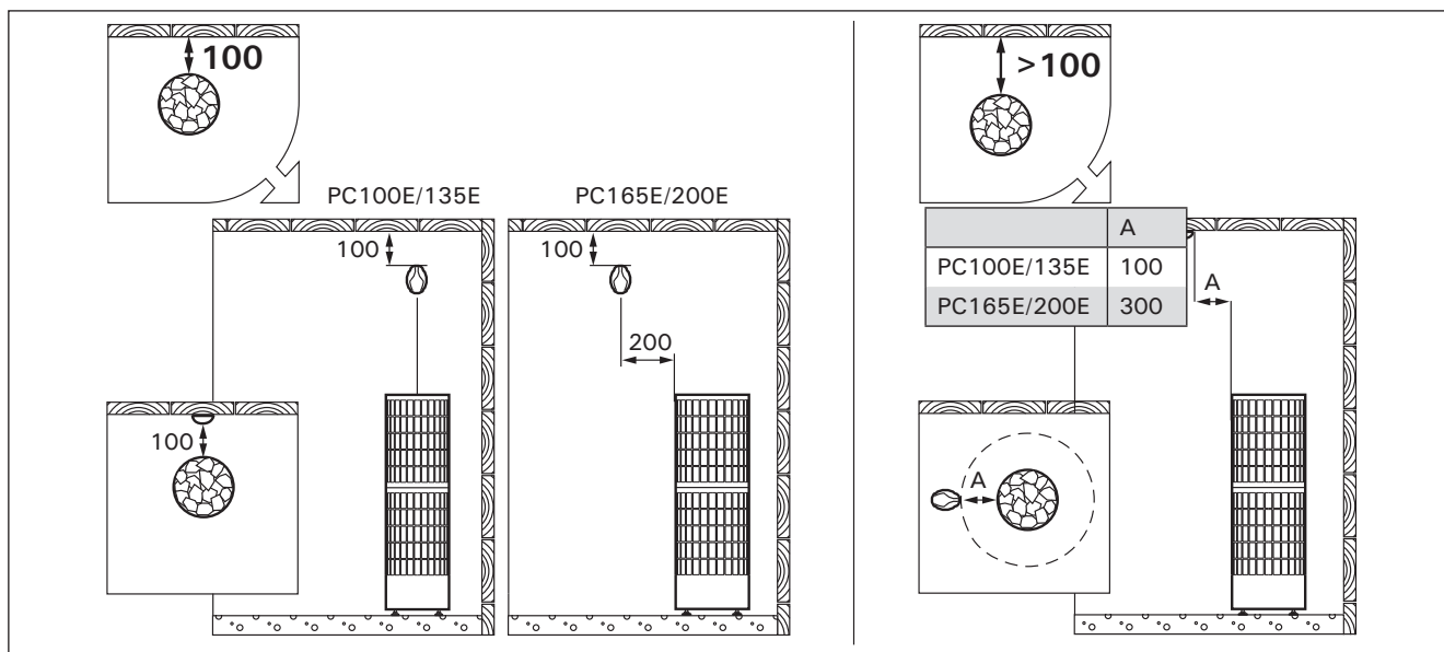
Installing the sensor (all dimensions in millimeters)
