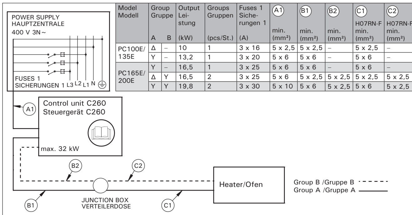
Electrical connections of control unit C260 and PC-E heater
