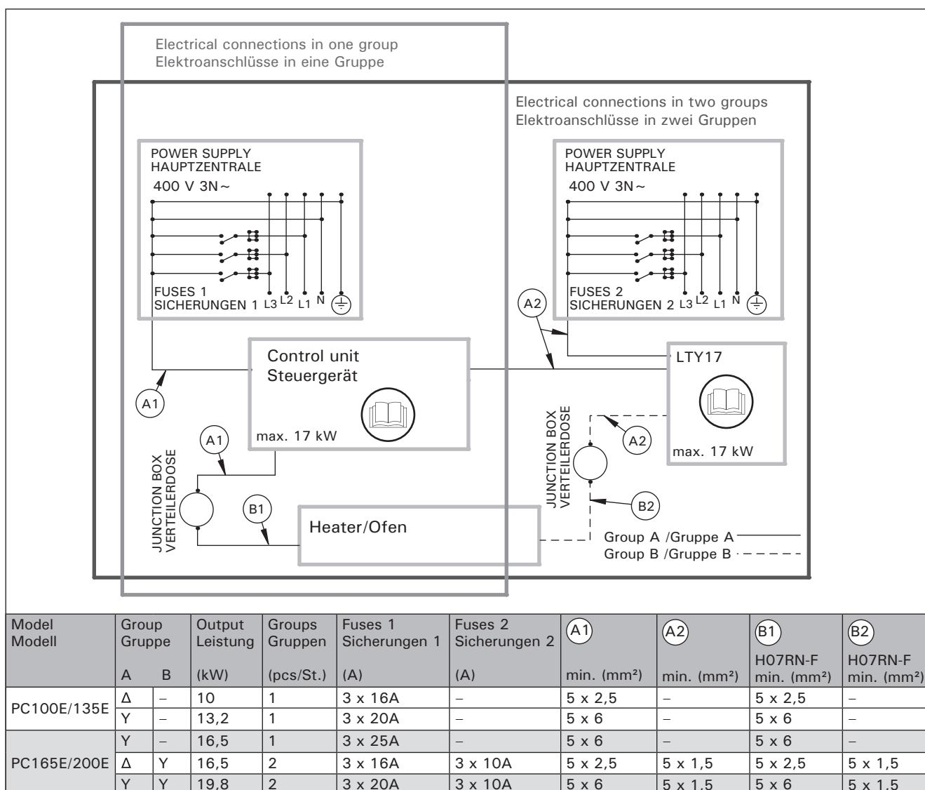
Electrical connections of control unit and PC-E heater
