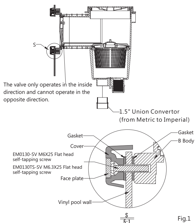
EM0130-SV, EM0130TS-SV INSTALLATION IN A VINYL POOL
