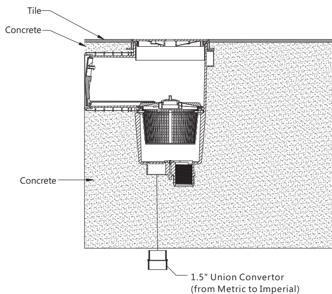
EM0130-SC INSTALLATION IN A CONCRETE POOL
