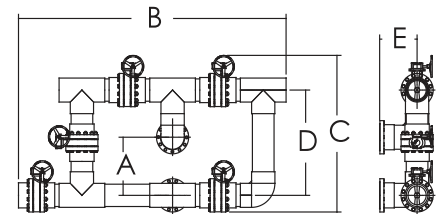
4 Way Butterfly Valve BVGT100- BVGT120
