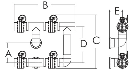
4 Way Butterfly Valve BVGT100- BVGT120
