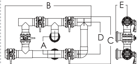
5 Way Butterfly Valve NBV30-NBV80
