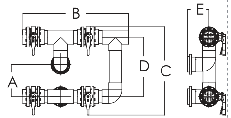
4 Way Butterfly Valve NBV30-NBV80
