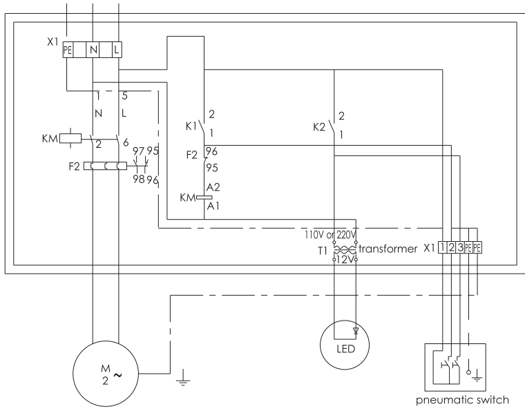
220V/50Hz, 110V/60Hz counter current jet circuit diagram
