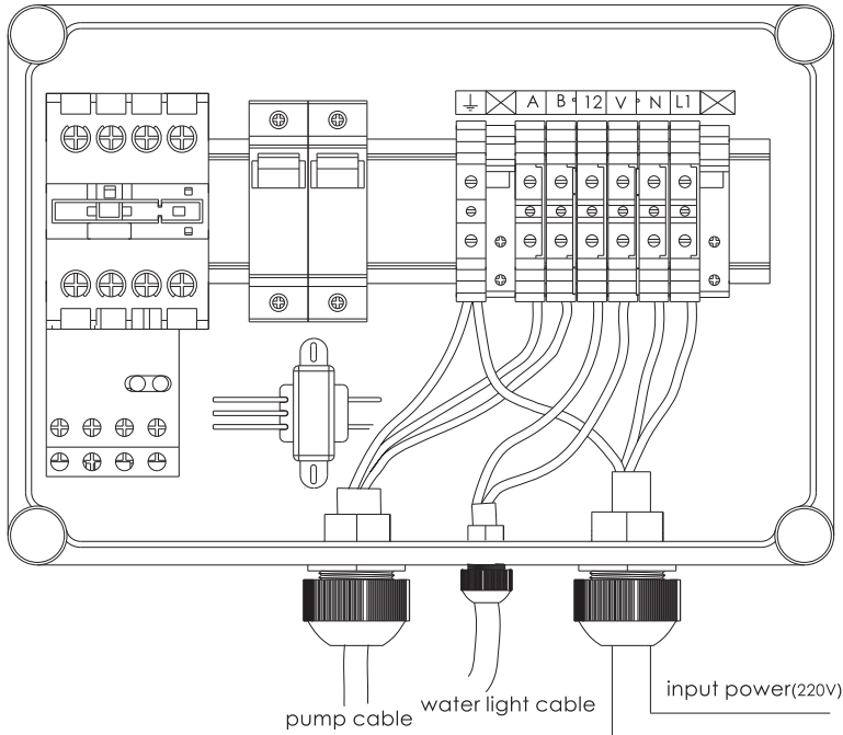
220V/110V control box wiring diagram
