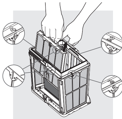
6.2.3 Continue to dismantle the panels in order: 2 → 3 → 4.
