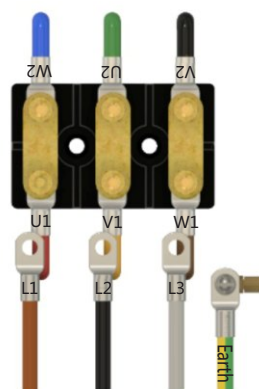
UPH550/UPH700 Delta Connection
