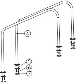
ANCHOR TYPE (ARN-F)
