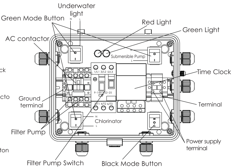
Small Control Box Diagram
