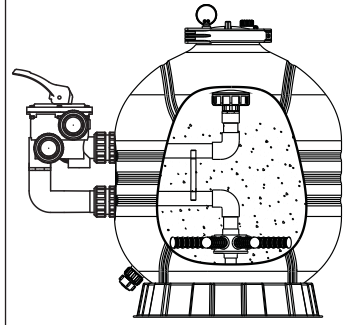
TYPICAL INSTALLATION
