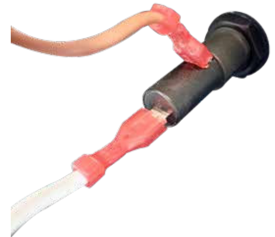
13 Fuse Holder
