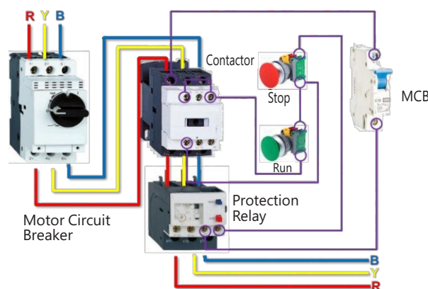
Direct-On-Line (DOL) Starter typical wiring.
