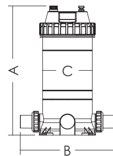
MODEL: CLL50 & CLL-75
