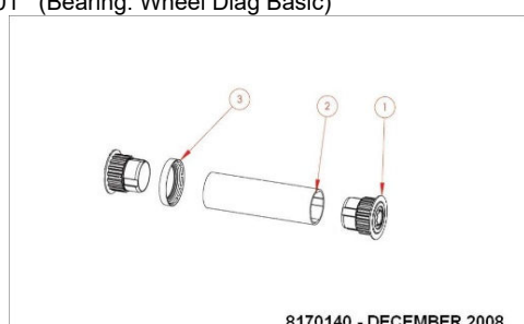
#01 (Bearing: Wheel Diag Basic)
