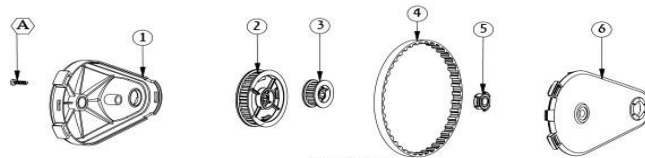
OPTION A WITH TRANSMISSION PULLIES
