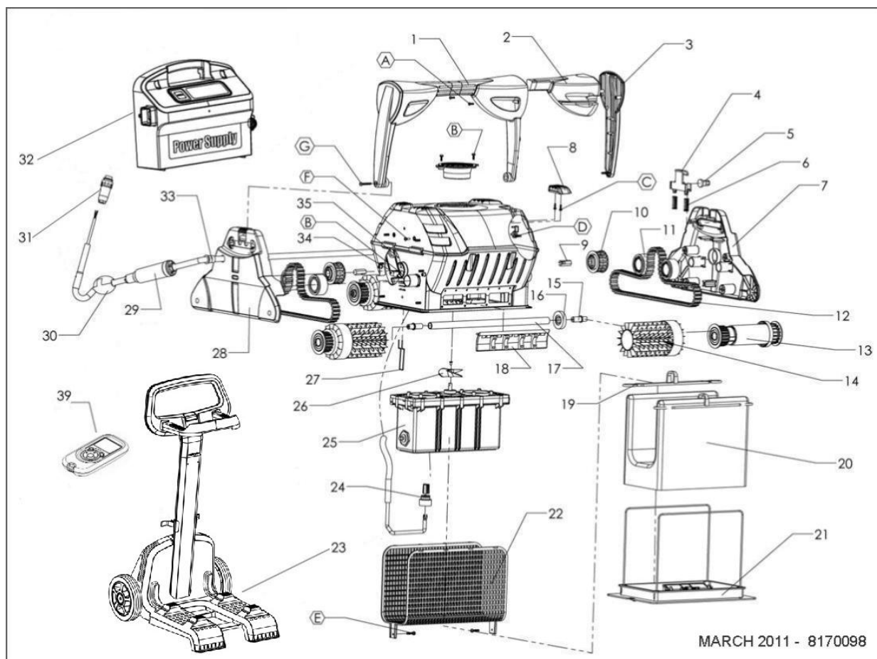
#01 (Handle Assy Wave 100)
