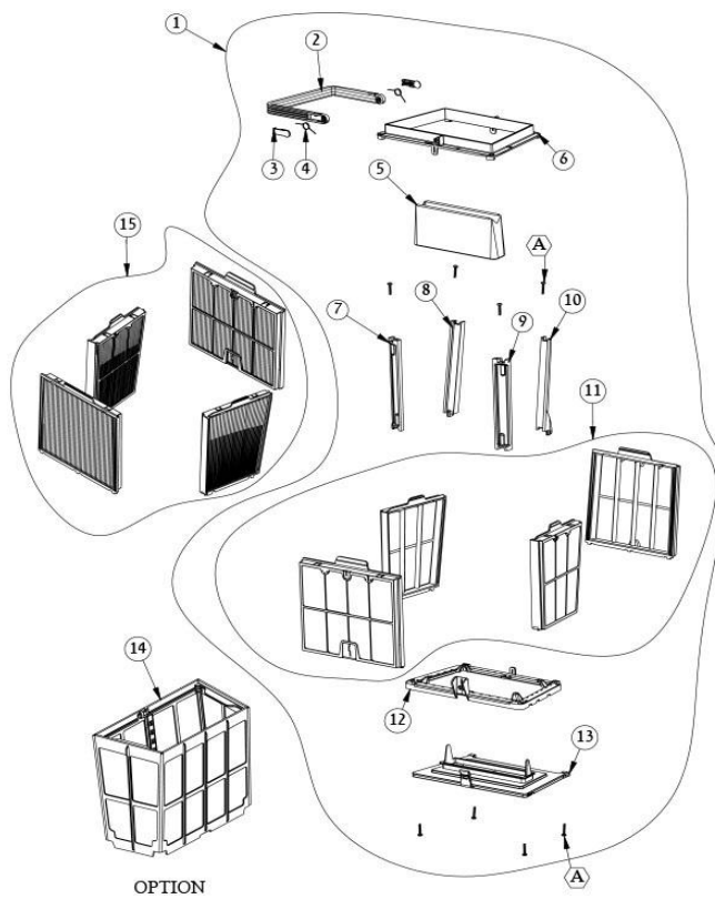
#01 (Filter Spring Filter Assy M2)
